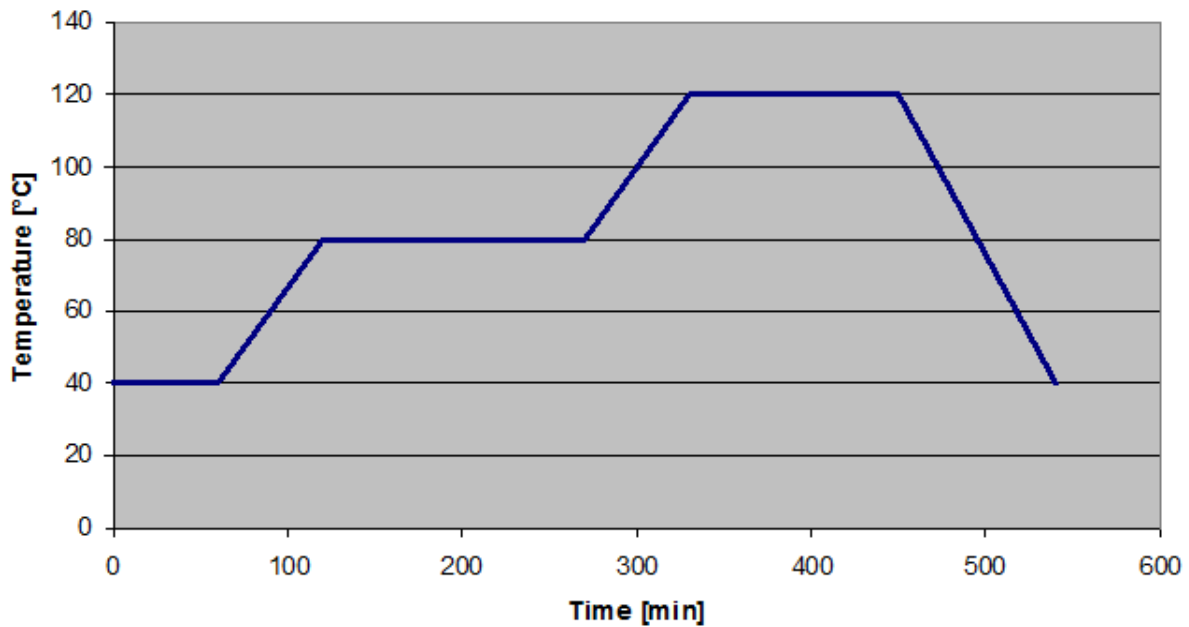
Proposed Cure Cycle for Part Thickness > 15 mm
