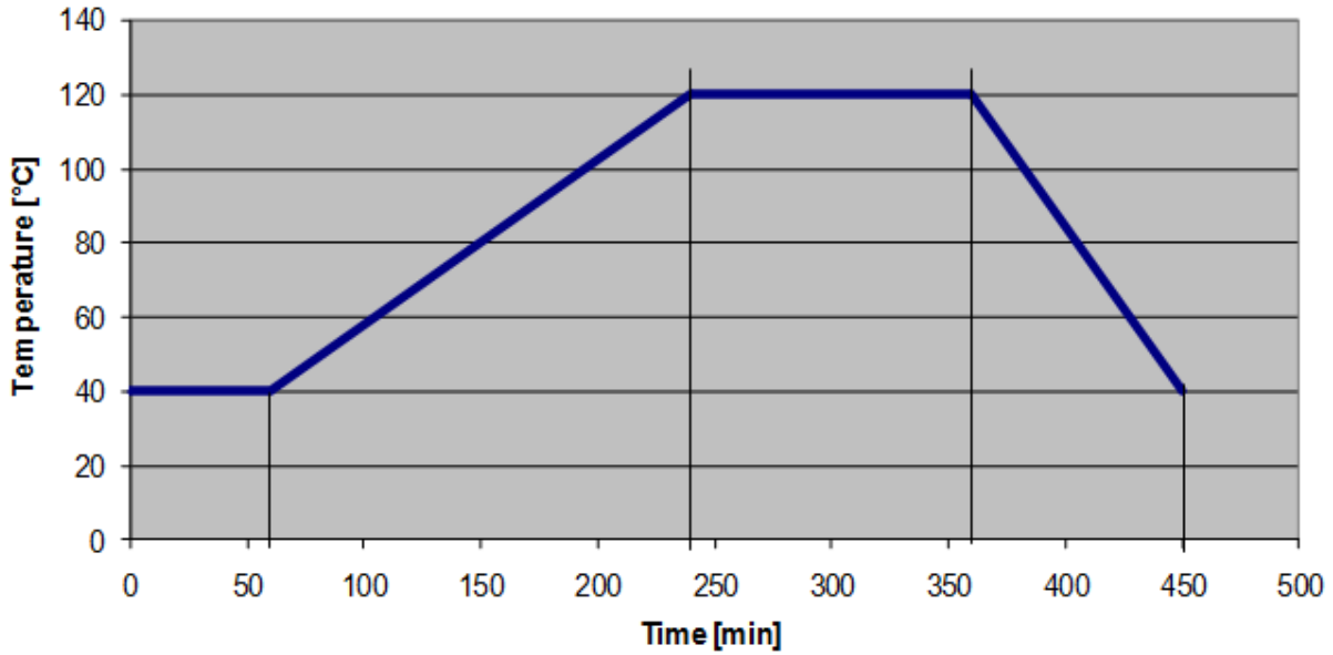
Proposed Cure Cycle for Part Thickness < 15 mm
